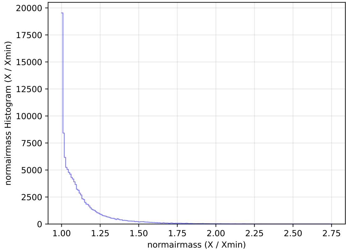
internal_u_expt45_nscale1.0v3.4_10yrs All sky u band: normairmass Histogram
