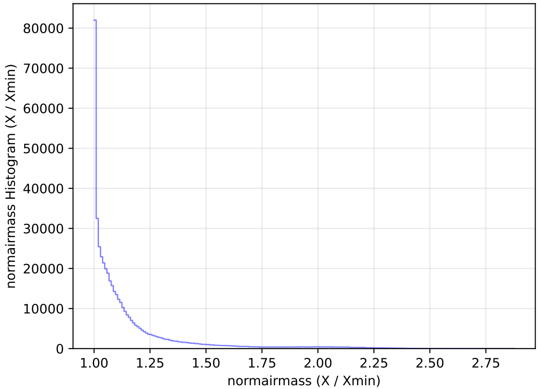
internal_u_expt45_nscale1.0v3.4_10yrs All sky r band: normairmass Histogram
