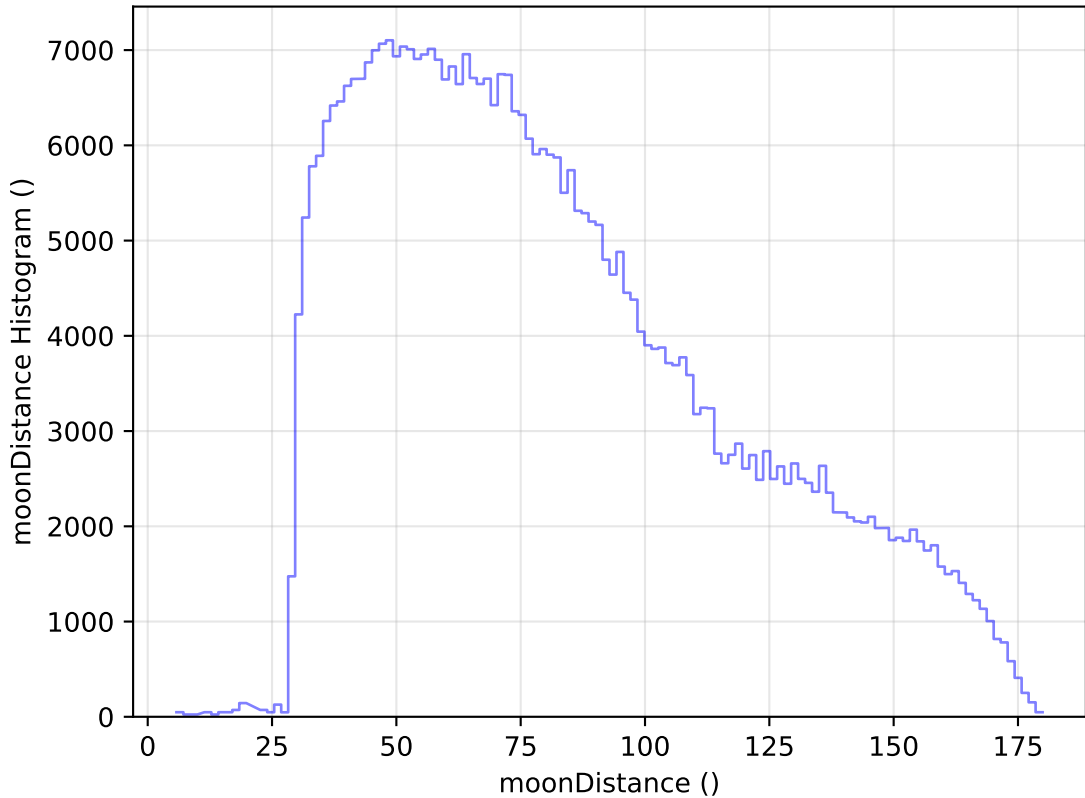
internal_u_expt45_nscale1.0v3.4_10yrs WFD z band: moonDistance Histogram
