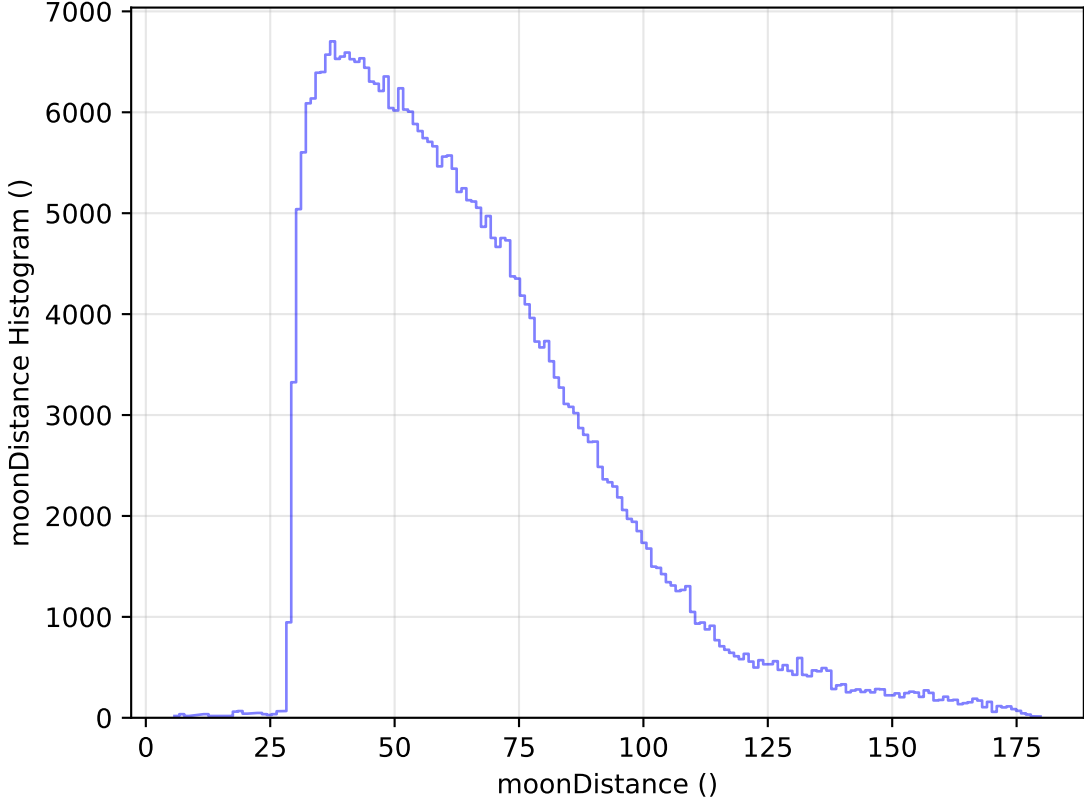
internal_u_expt45_nscale1.0v3.4_10yrs WFD y band: moonDistance Histogram
