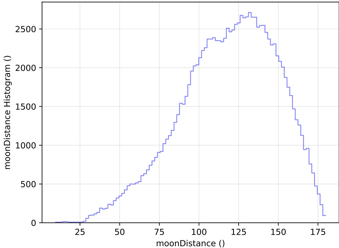
internal_u_expt45_nscale1.0v3.4_10yrs WFD u band: moonDistance Histogram
