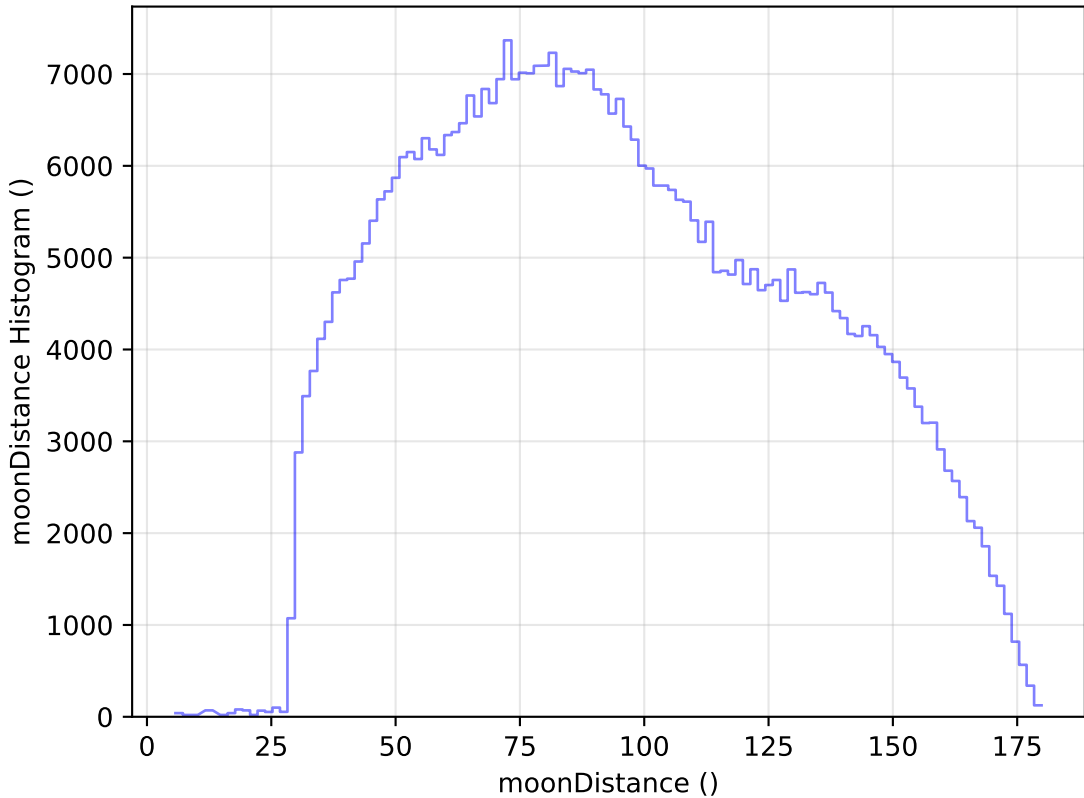
internal_u_expt45_nscale1.0v3.4_10yrs WFD i band: moonDistance Histogram
