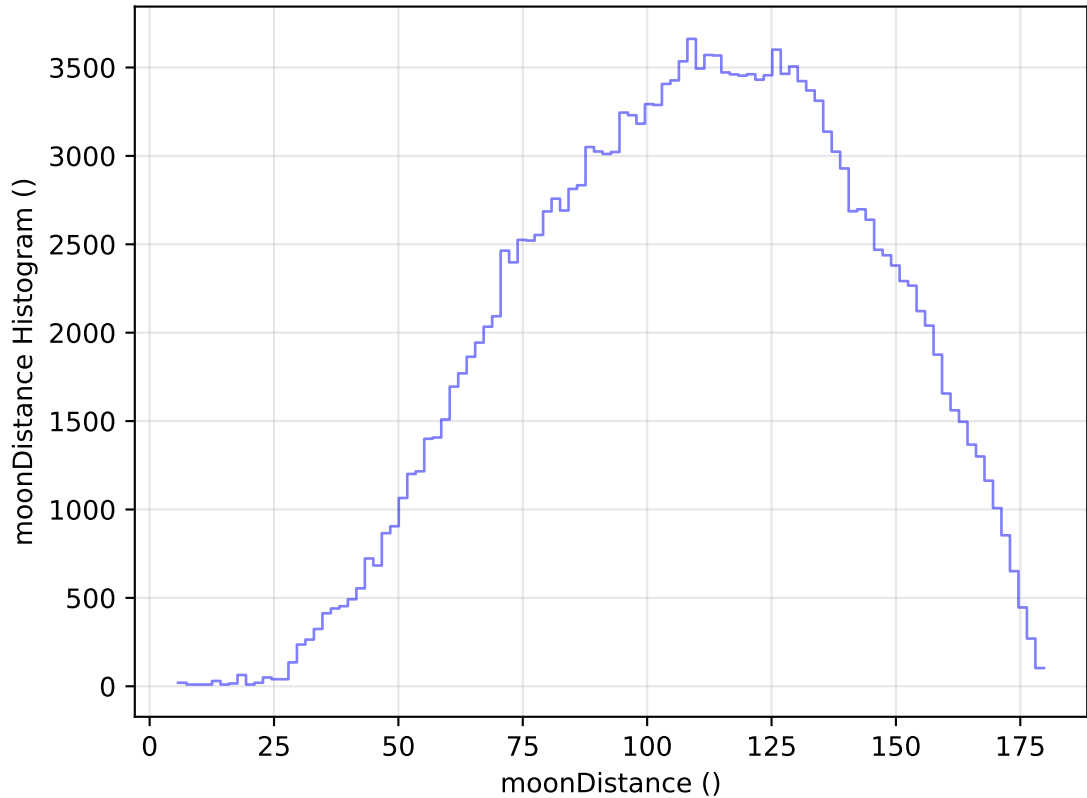
internal_u_expt45_nscale1.0v3.4_10yrs WFD g band: moonDistance Histogram
