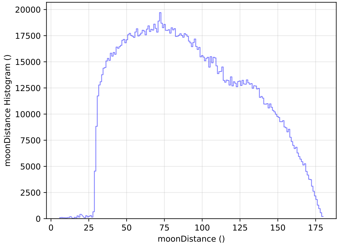
internal_u_expt45_nscale1.0v3.4_10yrs WFD all bands: moonDistance Histogram
