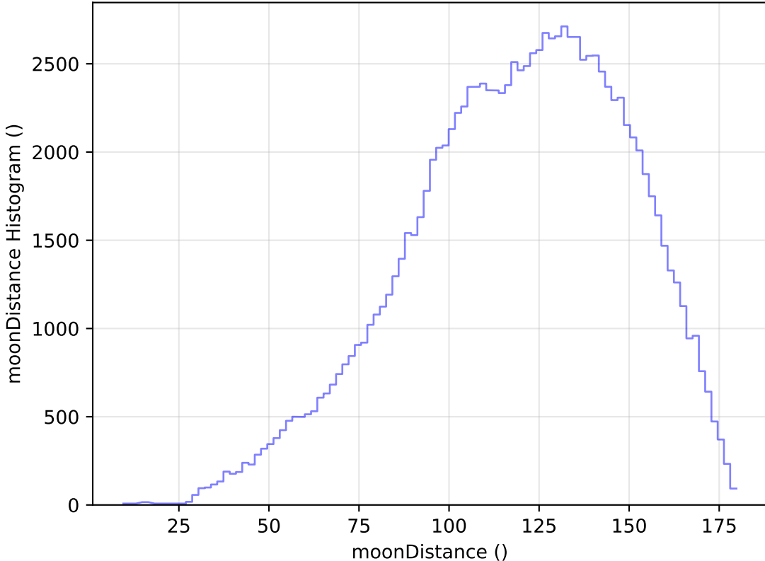
internal_u_expt45_nscale1.0v3.4_10yrs All sky u band: moonDistance Histogram
