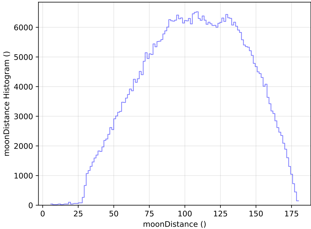
internal_u_expt45_nscale1.0v3.4_10yrs All sky r band: moonDistance Histogram
