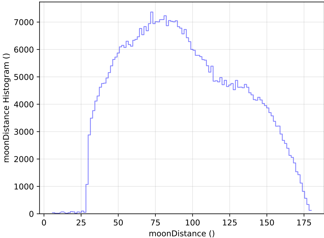
internal_u_expt45_nscale1.0v3.4_10yrs All sky i band: moonDistance Histogram
