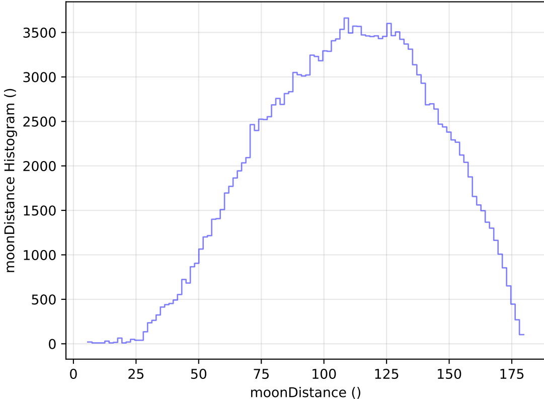
internal_u_expt45_nscale1.0v3.4_10yrs All sky g band: moonDistance Histogram
