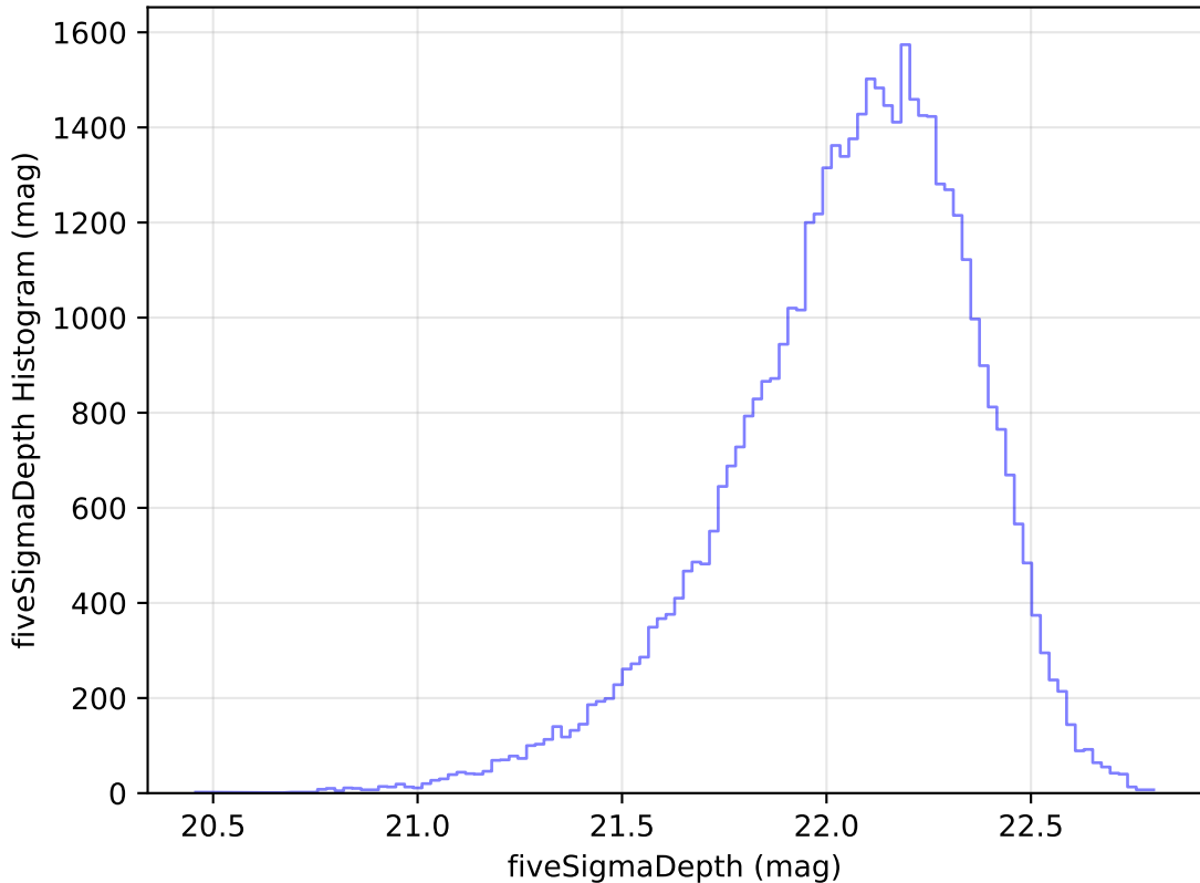
internal_u_expt45_nscale1.0v3.4_10yrs Yr 1 y band: fiveSigmaDepth Histogram
