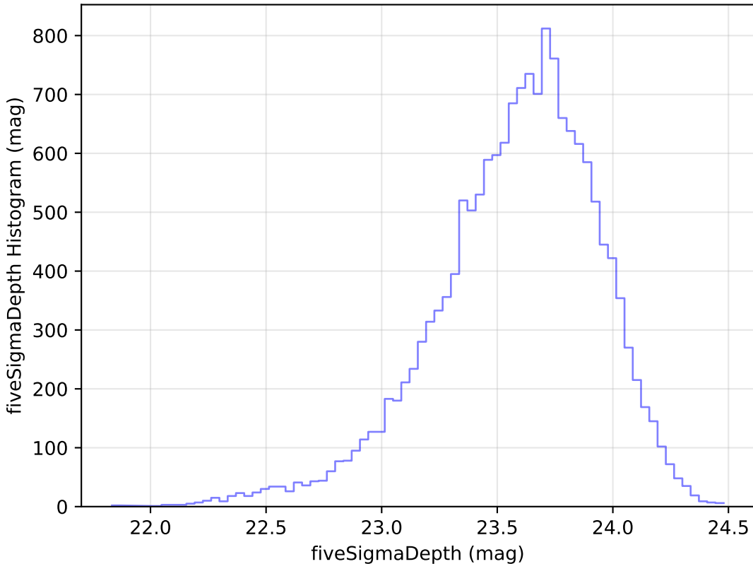
internal_u_expt45_nscale1.0v3.4_10yrs Yr 1 u band: fiveSigmaDepth Histogram
