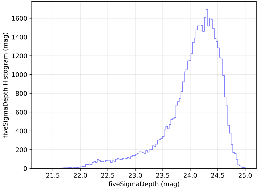
internal_u_expt45_nscale1.0v3.4_10yrs Yr 1 r band: fiveSigmaDepth Histogram
