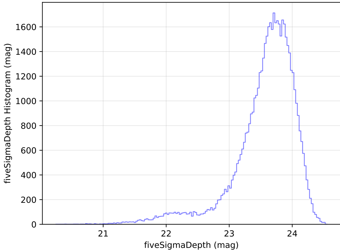
internal_u_expt45_nscale1.0v3.4_10yrs Yr 1 i band: fiveSigmaDepth Histogram
