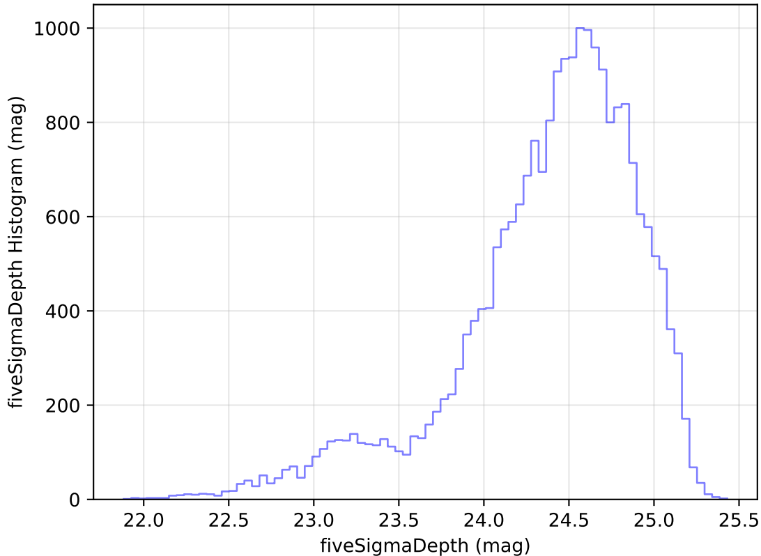
internal_u_expt45_nscale1.0v3.4_10yrs Yr 1 g band: fiveSigmaDepth Histogram
