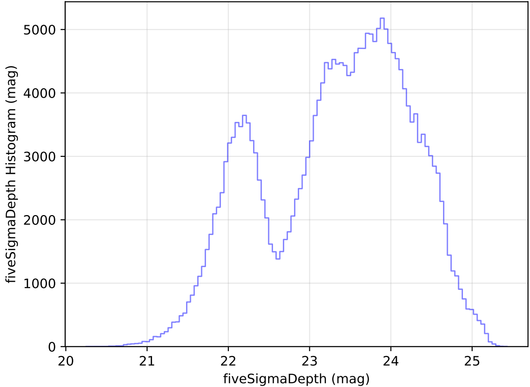
internal_u_expt45_nscale1.0v3.4_10yrs Yr 1 all bands: fiveSigmaDepth Histogram
