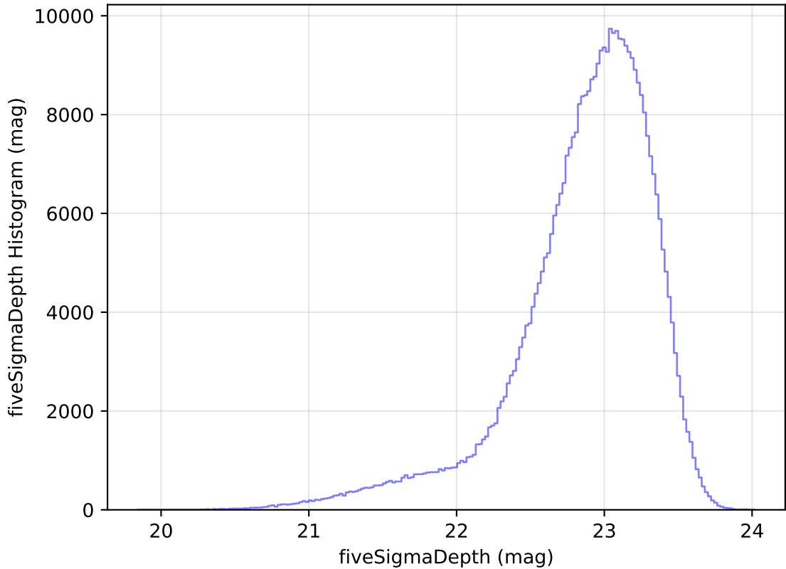
internal_u_expt45_nscale1.0v3.4_10yrs WFD z band: fiveSigmaDepth Histogram
