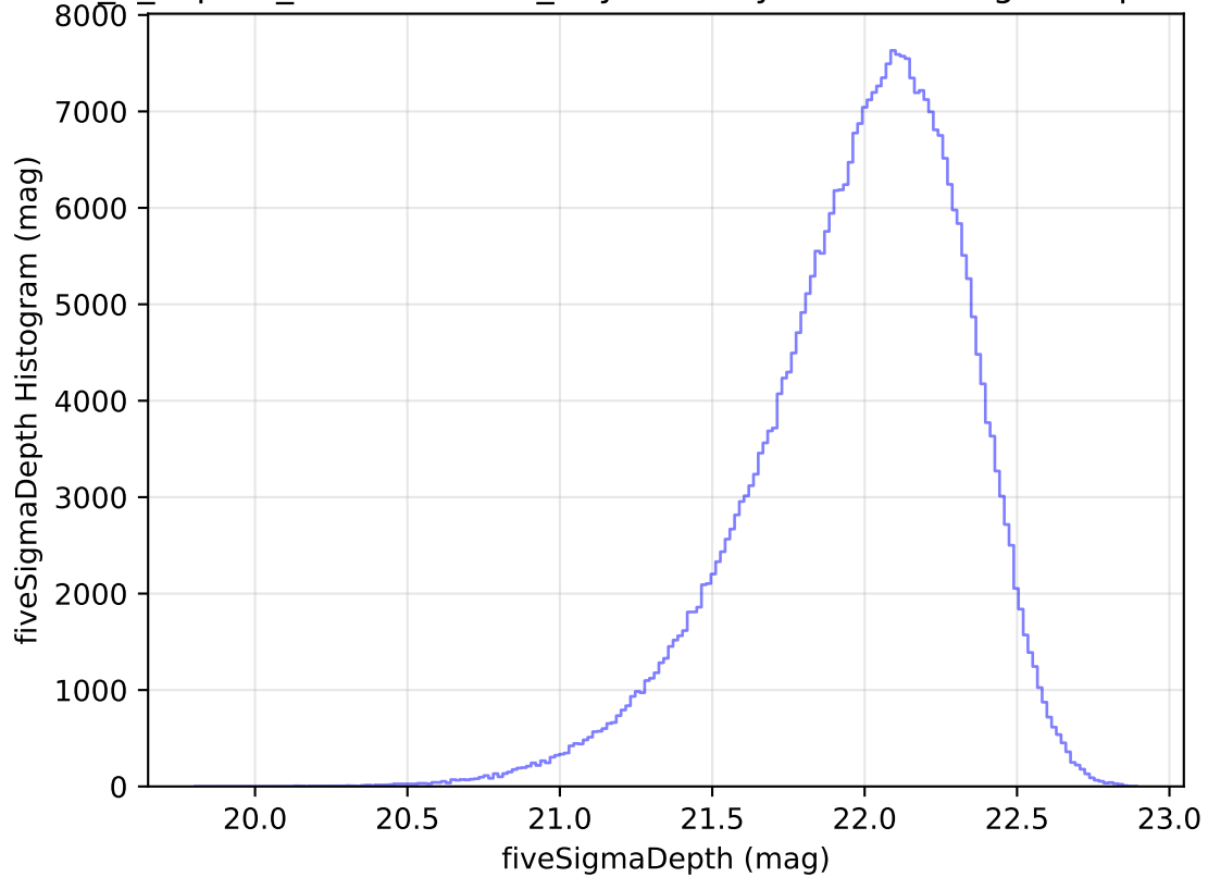
internal_u_expt45_nscale1.0v3.4_10yrs WFD y band: fiveSigmaDepth Histogram
