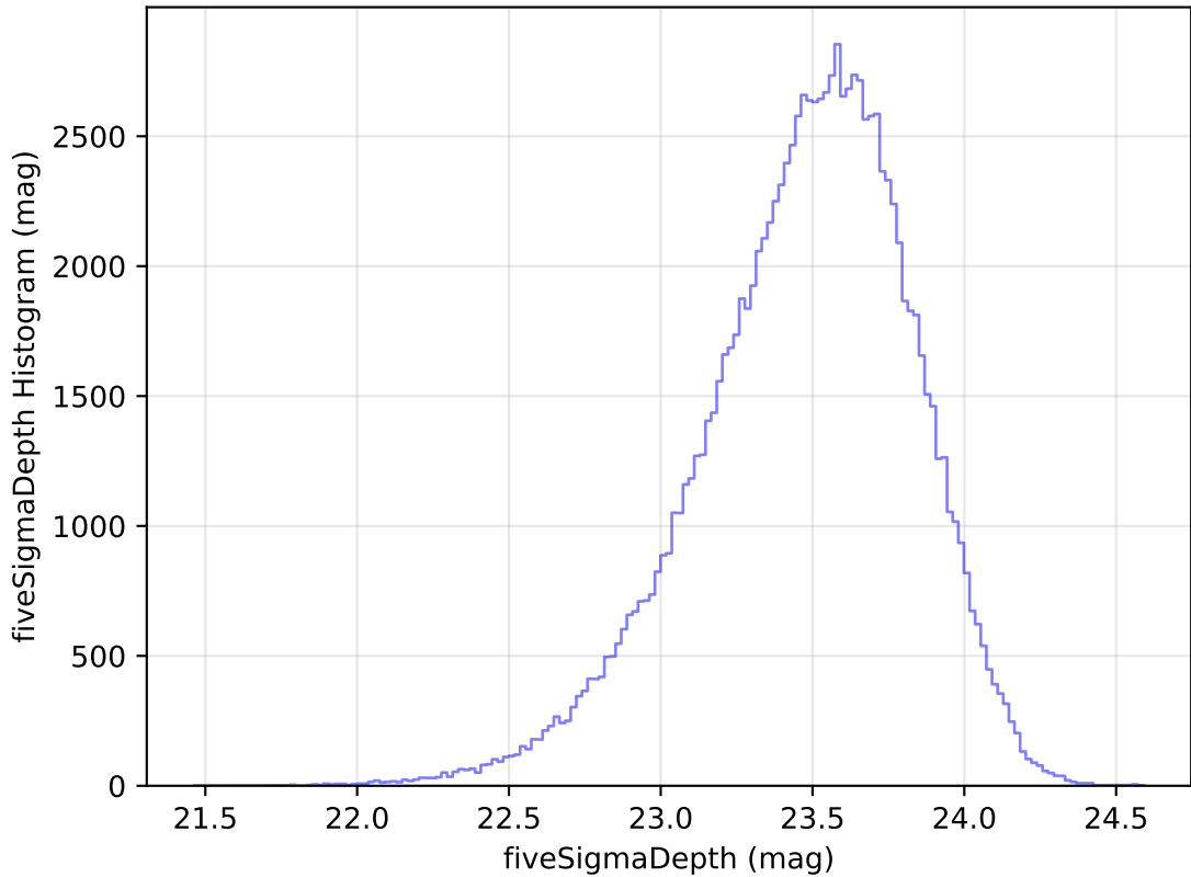
internal_u_expt45_nscale1.0v3.4_10yrs WFD u band: fiveSigmaDepth Histogram
