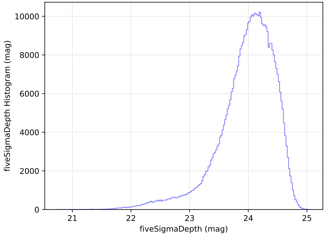
internal_u_expt45_nscale1.0v3.4_10yrs WFD r band: fiveSigmaDepth Histogram
