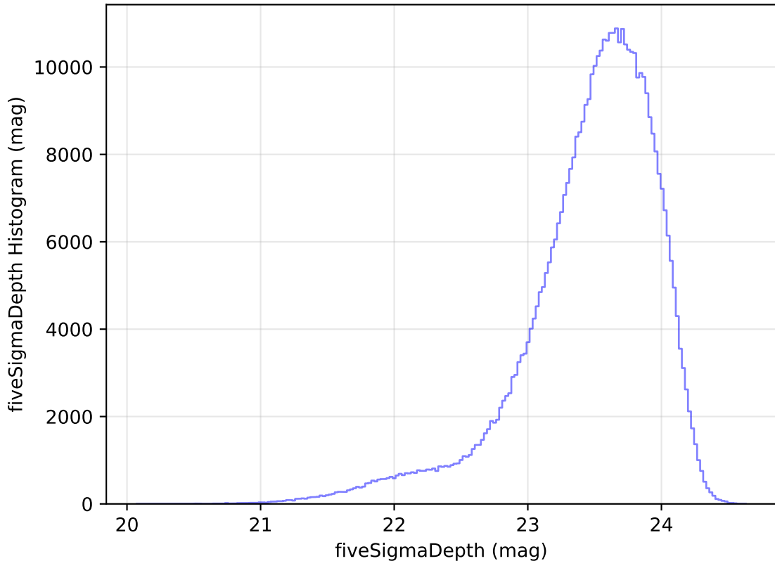
internal_u_expt45_nscale1.0v3.4_10yrs WFD i band: fiveSigmaDepth Histogram
