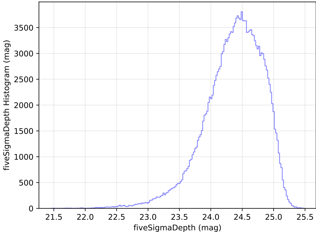
internal_u_expt45_nscale1.0v3.4_10yrs WFD g band: fiveSigmaDepth Histogram
