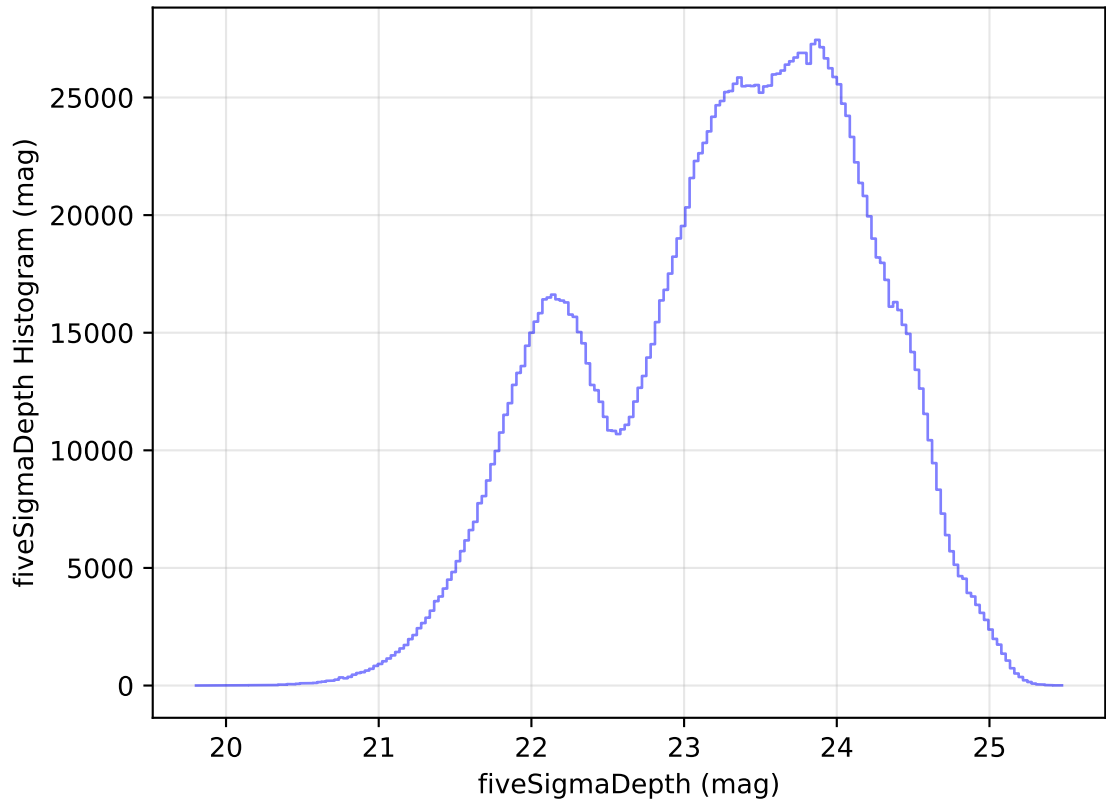
internal_u_expt45_nscale1.0v3.4_10yrs WFD all bands: fiveSigmaDepth Histogram
