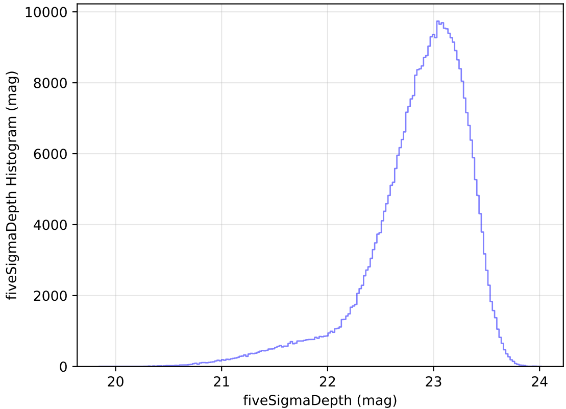
internal_u_expt45_nscale1.0v3.4_10yrs All sky z band: fiveSigmaDepth Histogram
