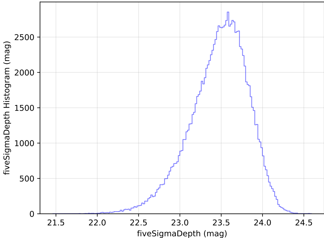
internal_u_expt45_nscale1.0v3.4_10yrs All sky u band: fiveSigmaDepth Histogram
