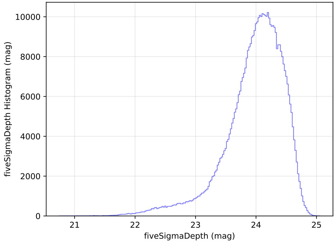
internal_u_expt45_nscale1.0v3.4_10yrs All sky r band: fiveSigmaDepth Histogram
