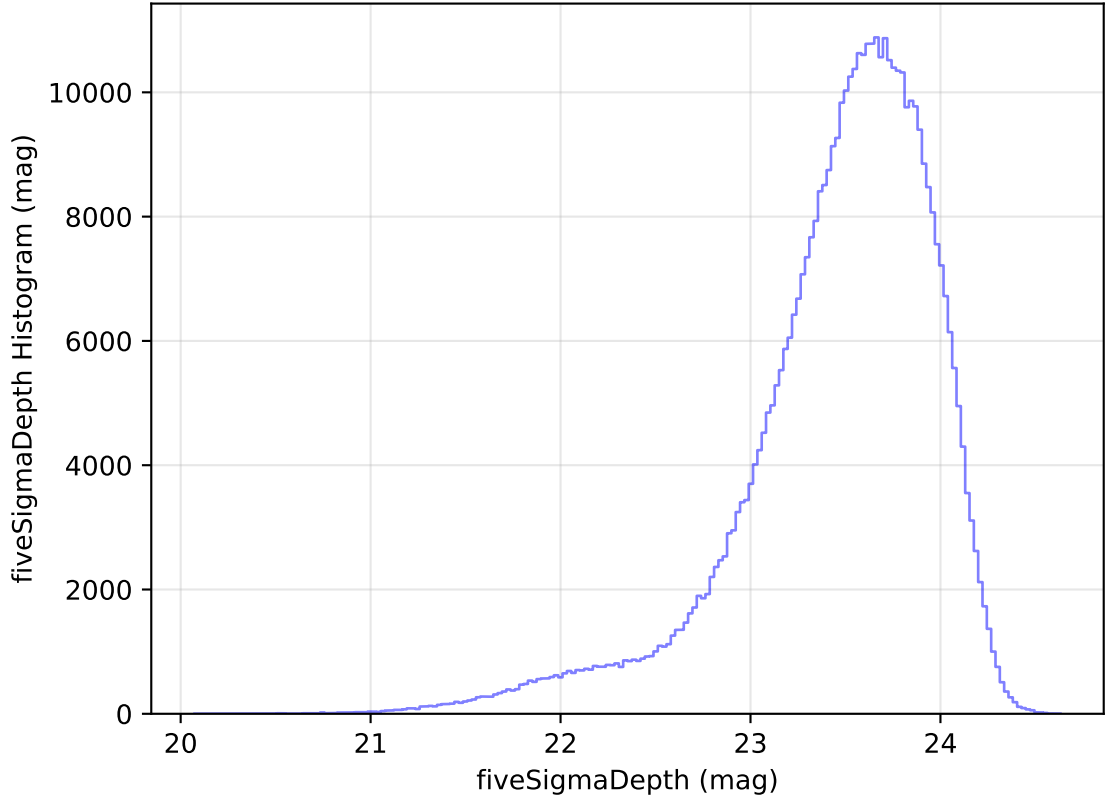
internal_u_expt45_nscale1.0v3.4_10yrs All sky i band: fiveSigmaDepth Histogram
