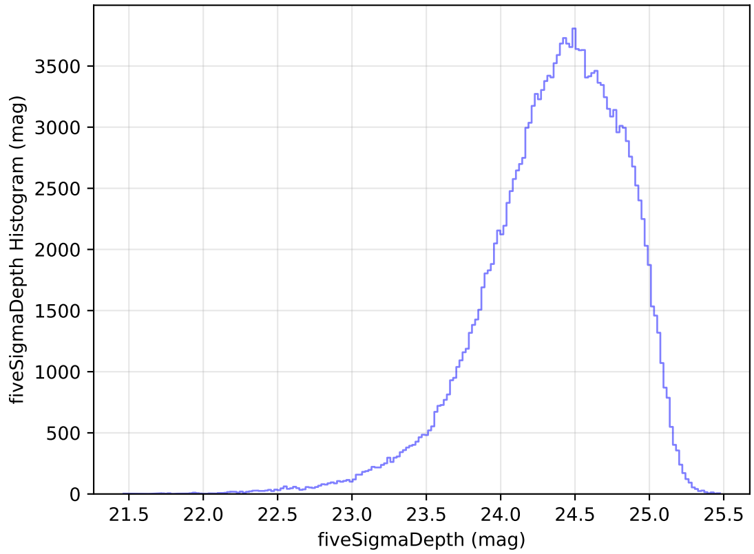
internal_u_expt45_nscale1.0v3.4_10yrs All sky g band: fiveSigmaDepth Histogram
