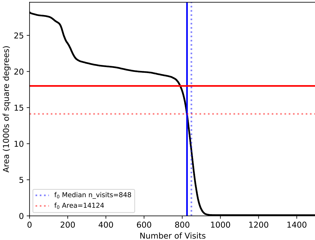
internal_u_expt45_nscale1.0v3.4_10yrs All sky: f0
