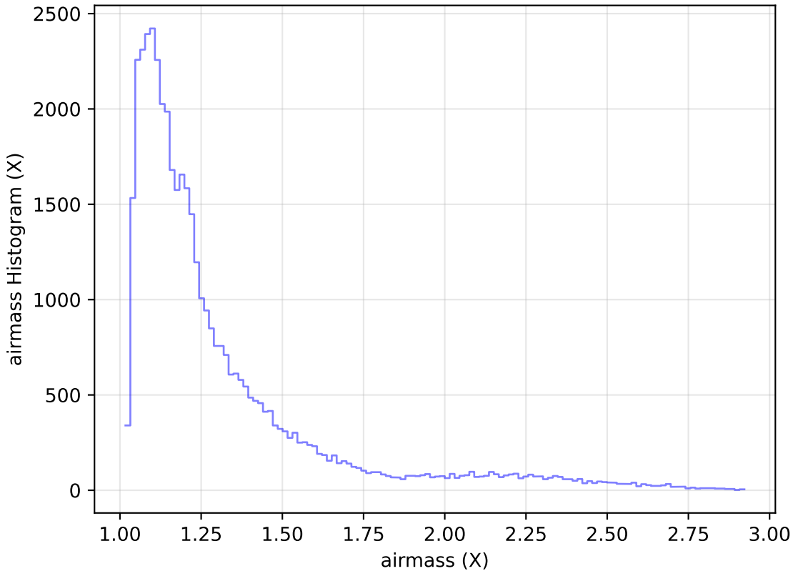
internal_u_expt45_nscale1.0v3.4_10yrs Yr 1 z band: airmass Histogram
