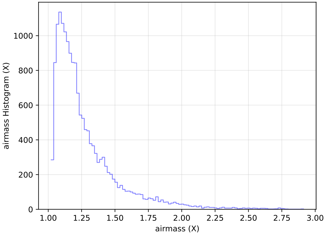
internal_u_expt45_nscale1.0v3.4_10yrs Yr 1 u band: airmass Histogram
