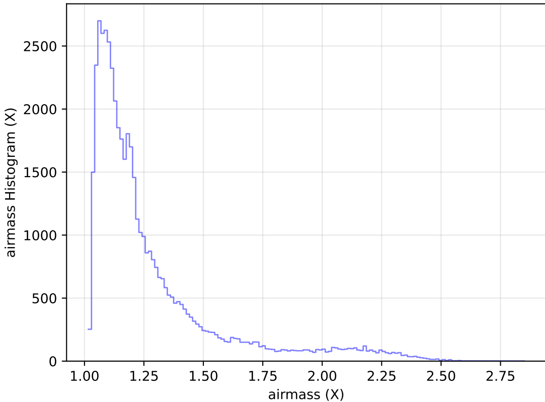
internal_u_expt45_nscale1.0v3.4_10yrs Yr 1 r band: airmass Histogram
