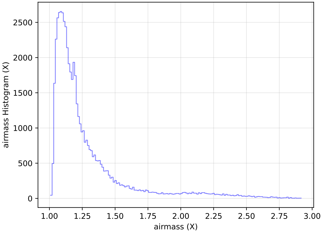
internal_u_expt45_nscale1.0v3.4_10yrs Yr 1 i band: airmass Histogram
