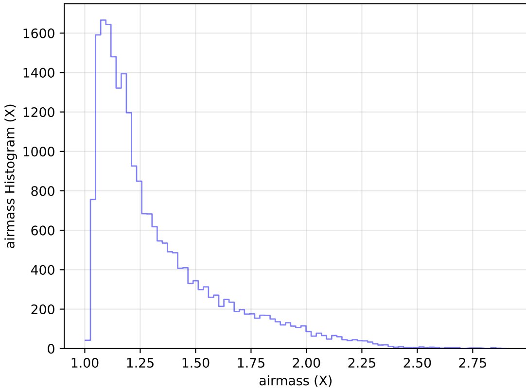
internal_u_expt45_nscale1.0v3.4_10yrs Yr 1 g band: airmass Histogram
