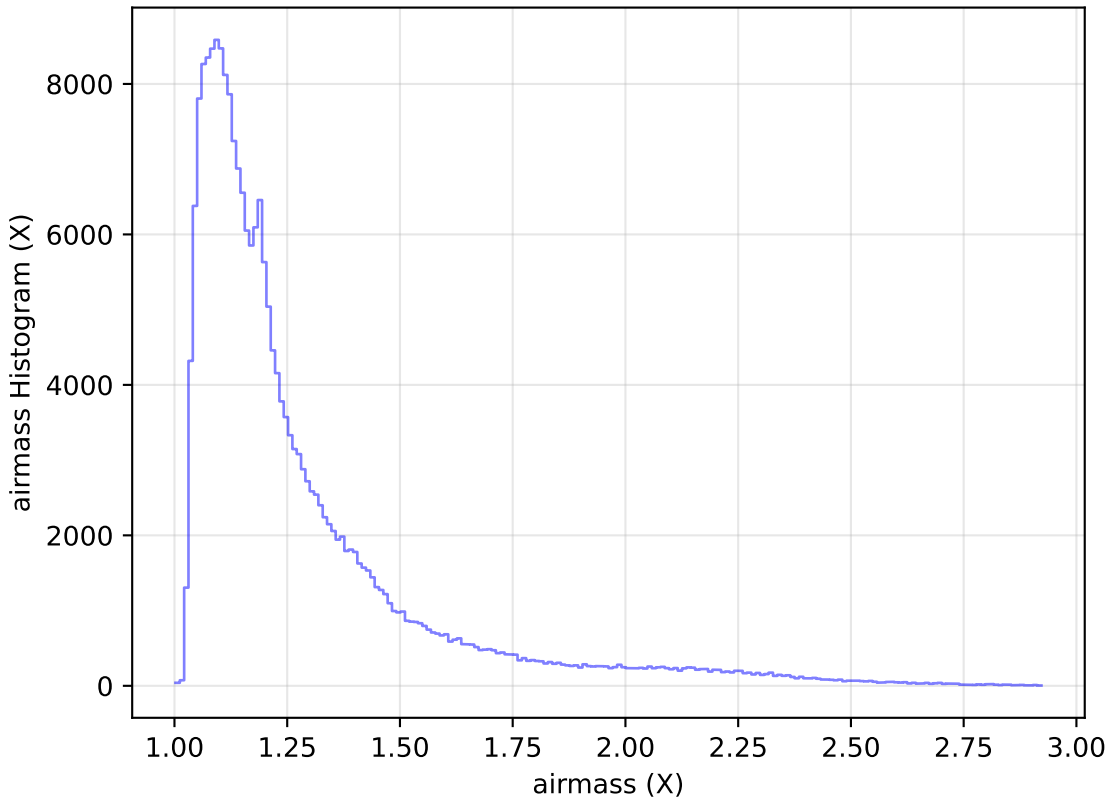
internal_u_expt45_nscale1.0v3.4_10yrs Yr 1 all bands: airmass Histogram
