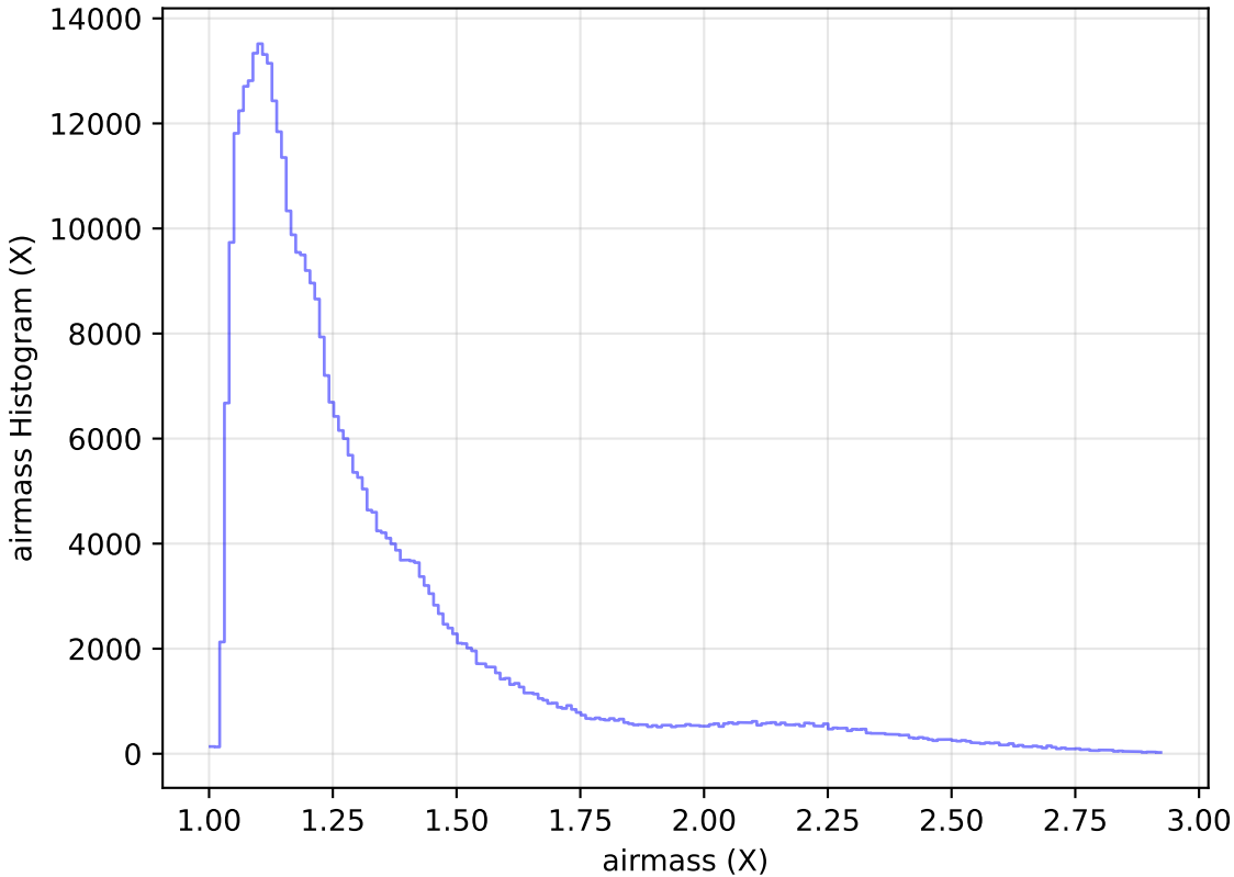
internal_u_expt45_nscale1.0v3.4_10yrs WFD z band: airmass Histogram
