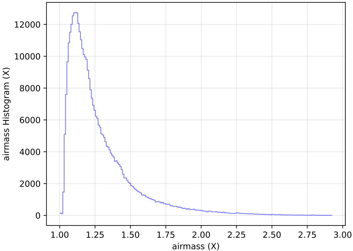
internal_u_expt45_nscale1.0v3.4_10yrs WFD y band: airmass Histogram
