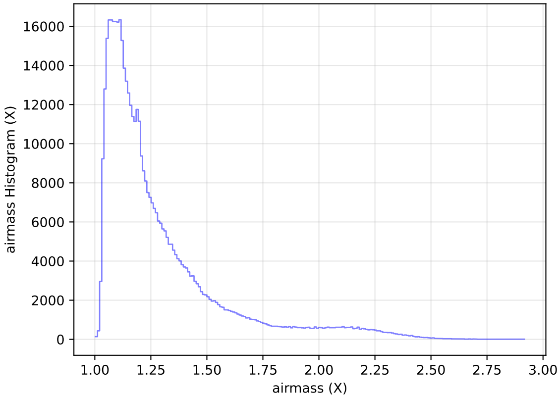
internal_u_expt45_nscale1.0v3.4_10yrs WFD r band: airmass Histogram
