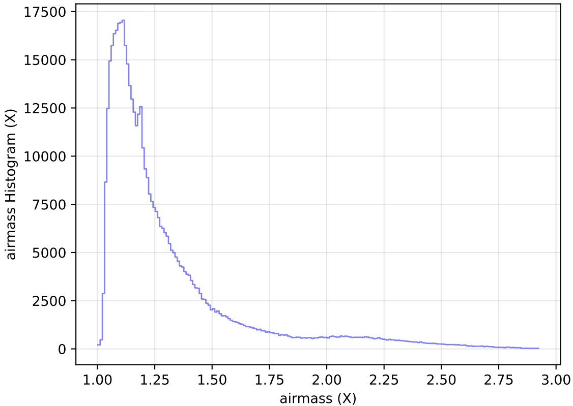
internal_u_expt45_nscale1.0v3.4_10yrs WFD i band: airmass Histogram
