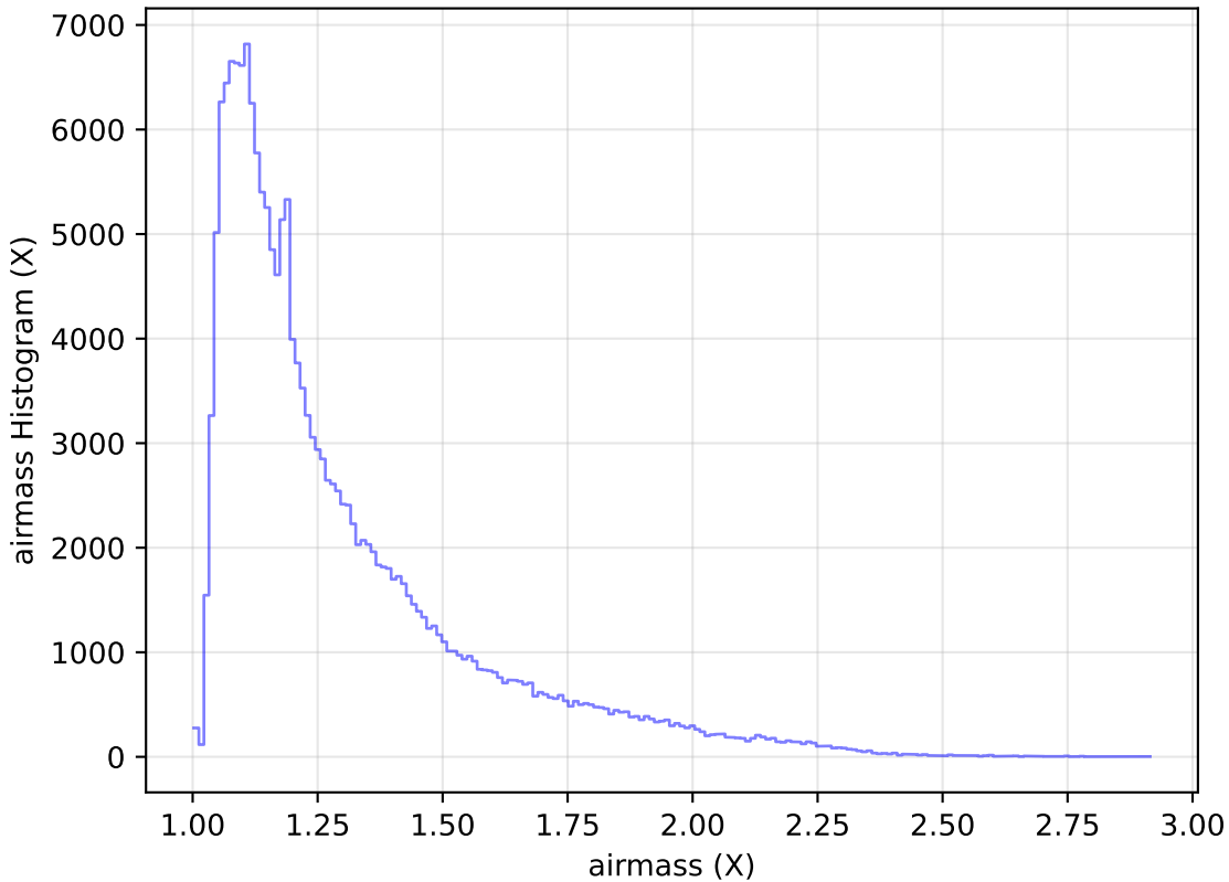
internal_u_expt45_nscale1.0v3.4_10yrs WFD g band: airmass Histogram
