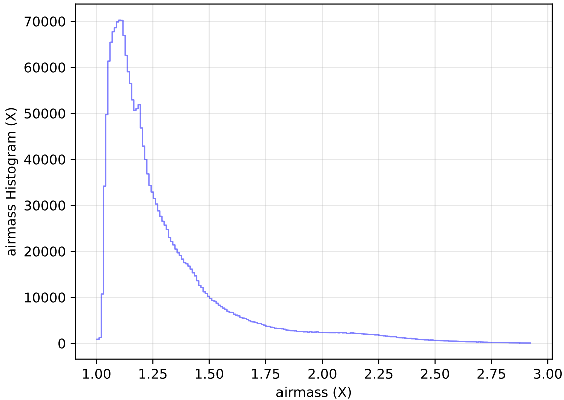
internal_u_expt45_nscale1.0v3.4_10yrs WFD all bands: airmass Histogram
