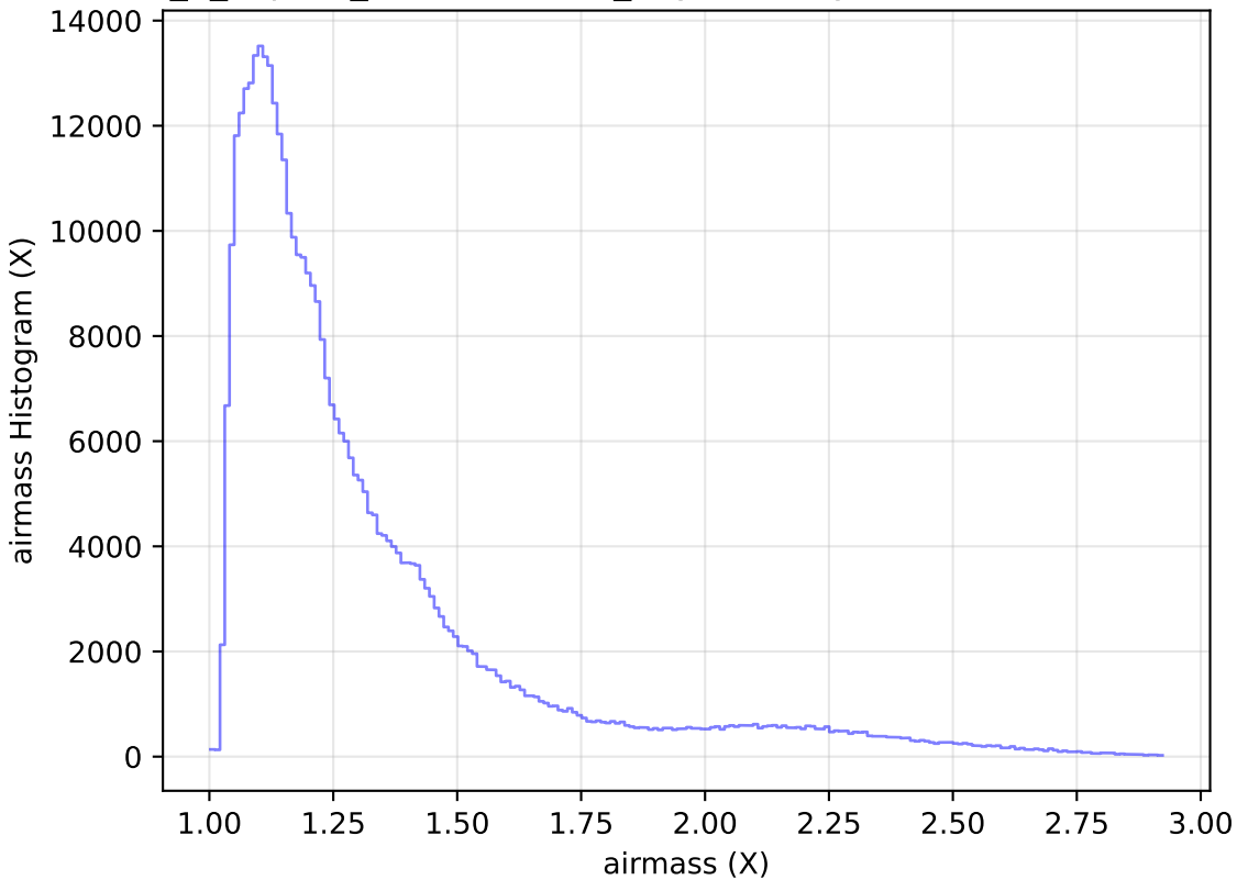
internal_u_expt45_nscale1.0v3.4_10yrs All sky z band: airmass Histogram
