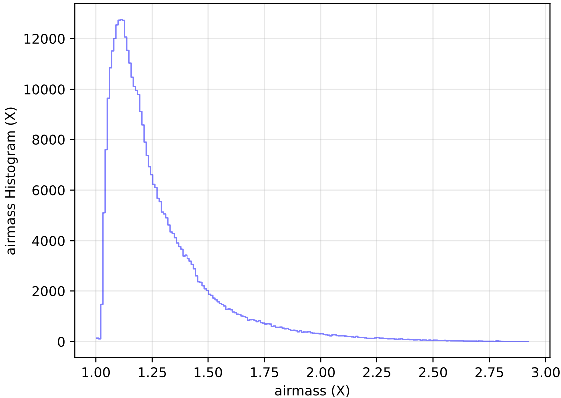
internal_u_expt45_nscale1.0v3.4_10yrs All sky y band: airmass Histogram
