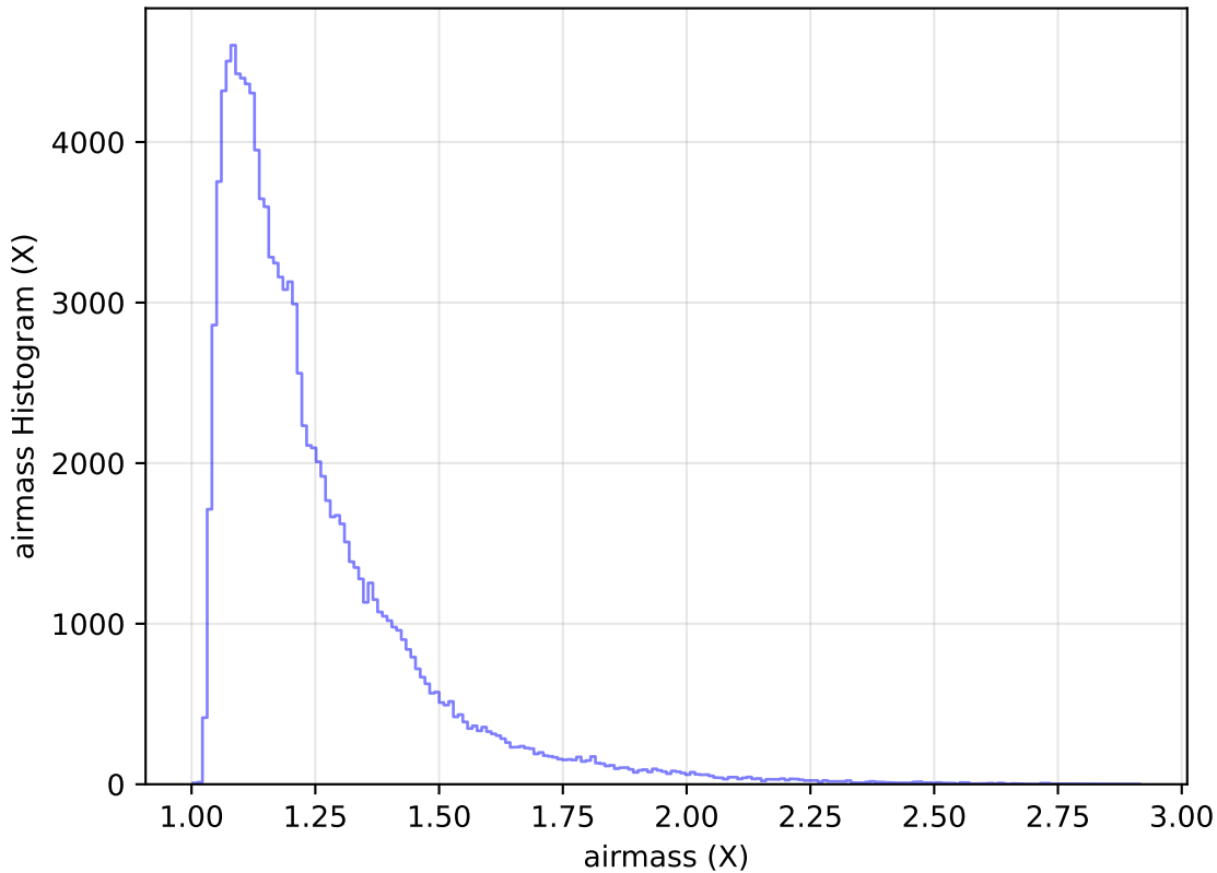
internal_u_expt45_nscale1.0v3.4_10yrs All sky u band: airmass Histogram
