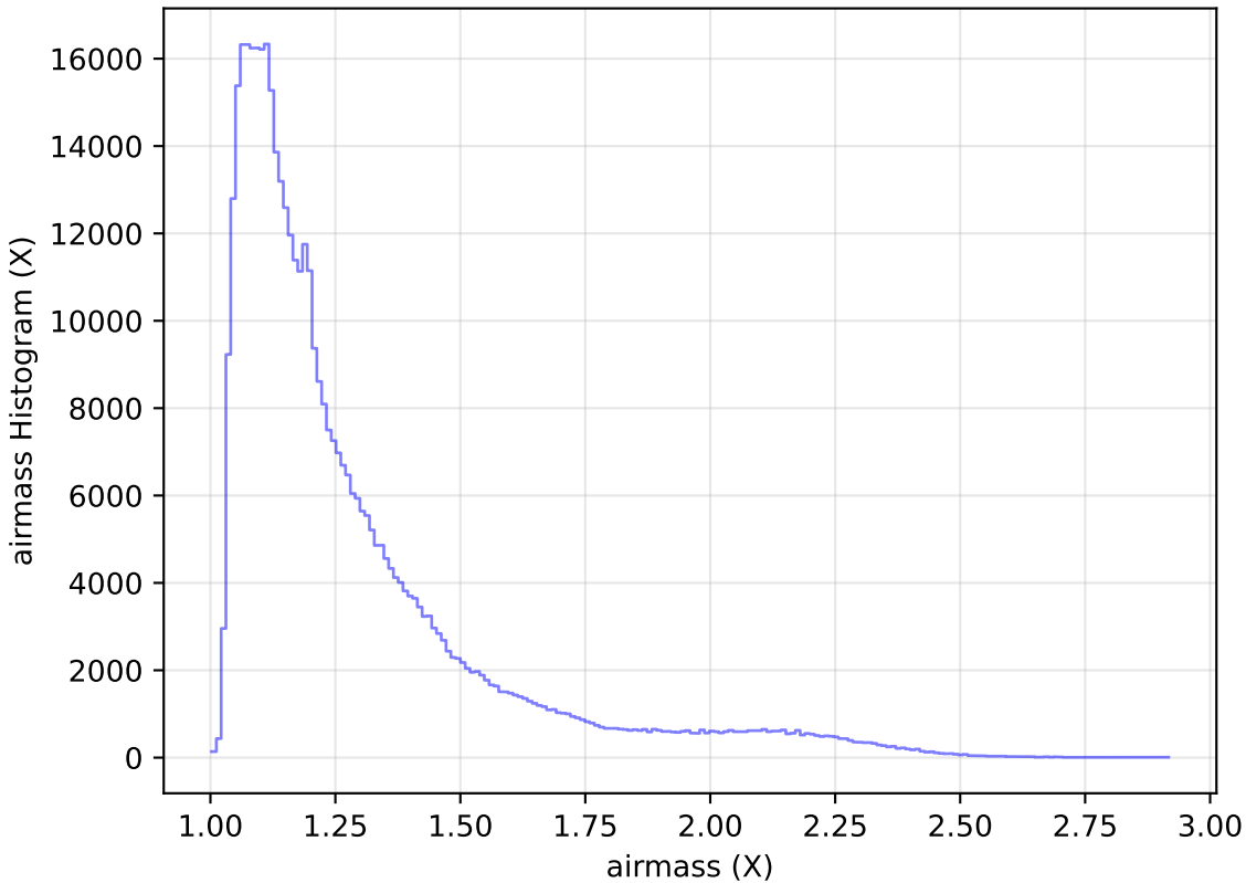
internal_u_expt45_nscale1.0v3.4_10yrs All sky r band: airmass Histogram
