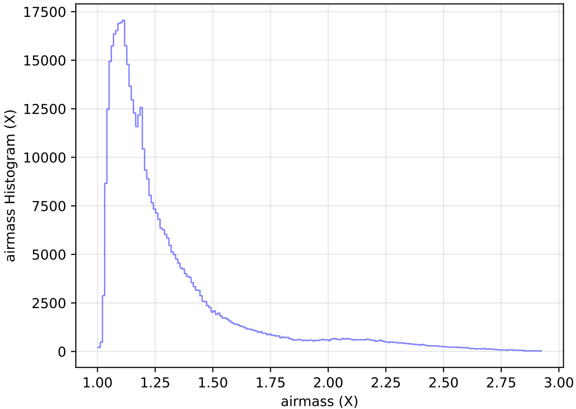
internal_u_expt45_nscale1.0v3.4_10yrs All sky i band: airmass Histogram
