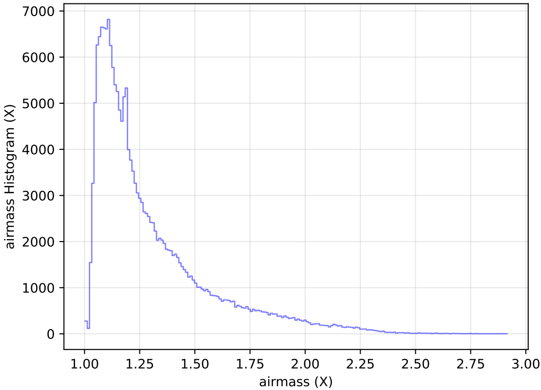
internal_u_expt45_nscale1.0v3.4_10yrs All sky g band: airmass Histogram
