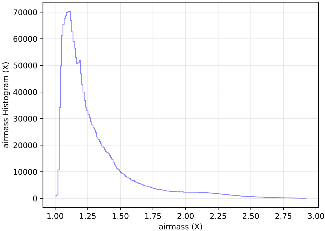
internal_u_expt45_nscale1.0v3.4_10yrs All sky all bands: airmass Histogram
